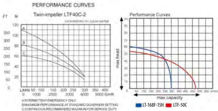
LTF40C-2 (2 IMPELLER)
